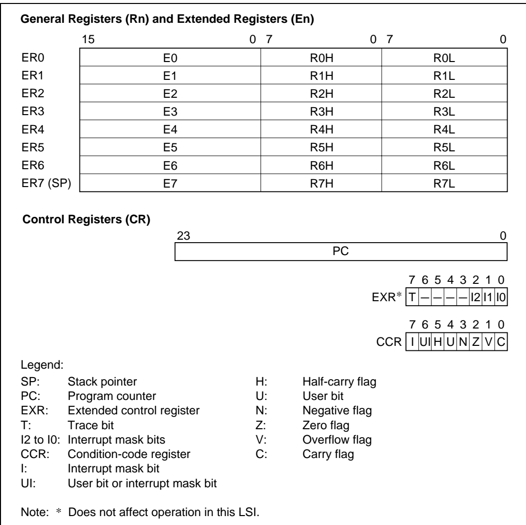
Figure 2.7 CPU Registers
