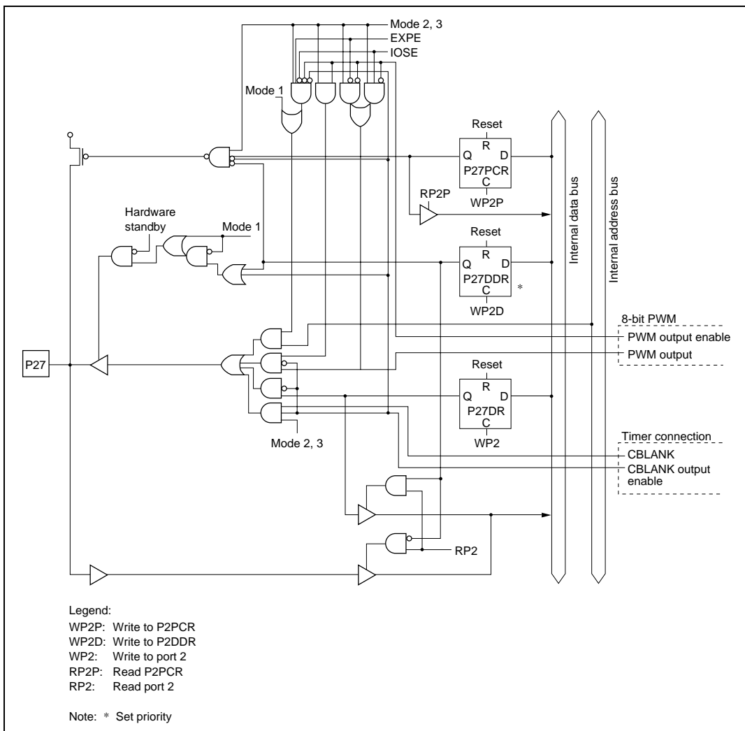
Figure C.4 Port 2 Block Diagram (Pin P27)
